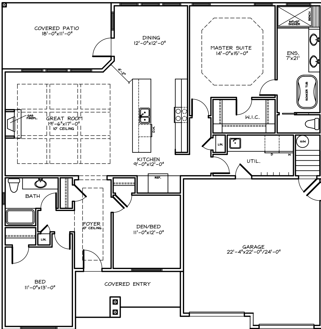
MAIN FLOOR PLAN 1885 SQ. FT.
